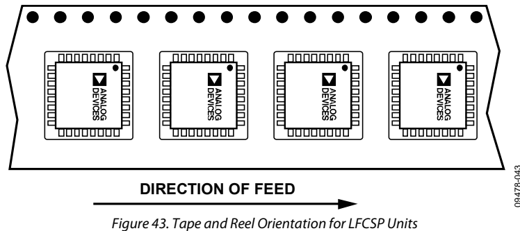
Figure 43. Tape and Reel Orientation for LFCSP Units
