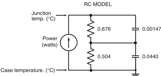
FIGURE 25b. TRANSIENT THERMAL IMPEDANCE MODEL
