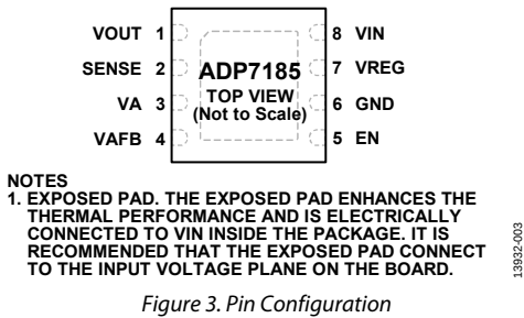
Figure 3. Pin Configuration
