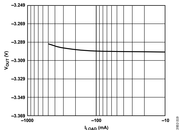
Figure 19. Output Voltage ( V_{OUT} ) vs. Load Current ( I_{LOAD} ), V_{OUT} = -3.3 V
