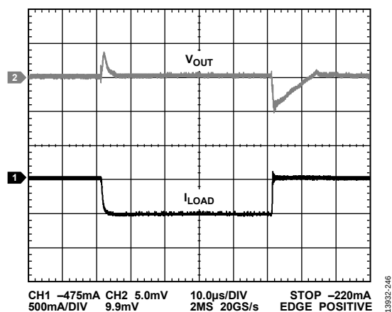
Figure 46. Output Transient Response, C_{\text{OUT}} = 4.7 \mu\text{F} , V_{\text{OUT}} = -1.2 \text{ V}
