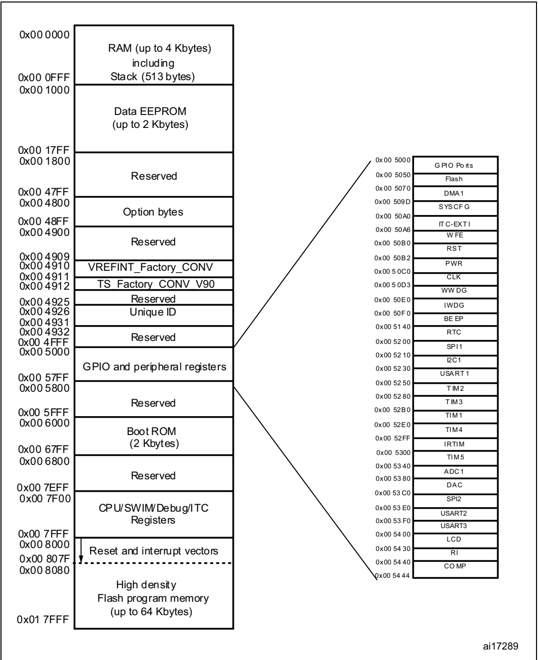
Figure 10. Memory map
