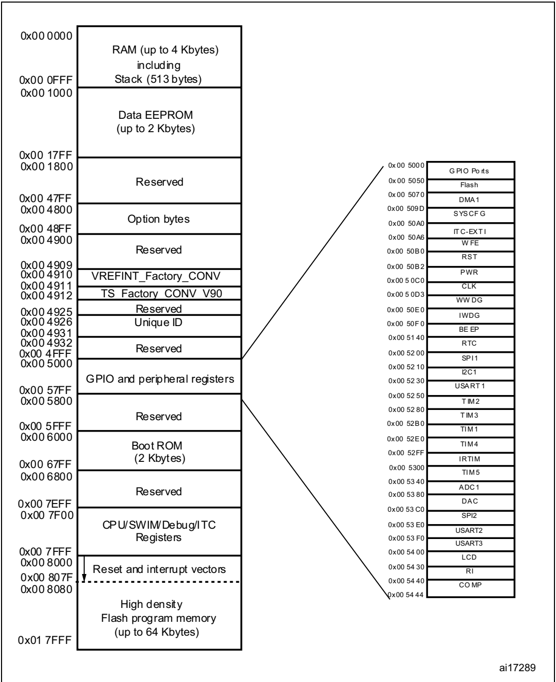
Figure 10. Memory map
