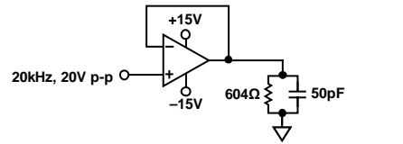
Figure 28. Output Swing, Vs = ±15V, G = +1
