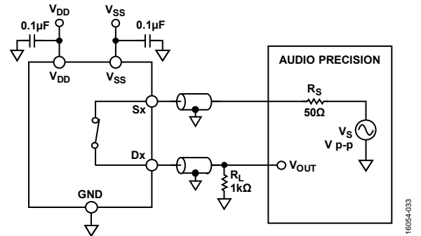
Figure 33. THD + N
