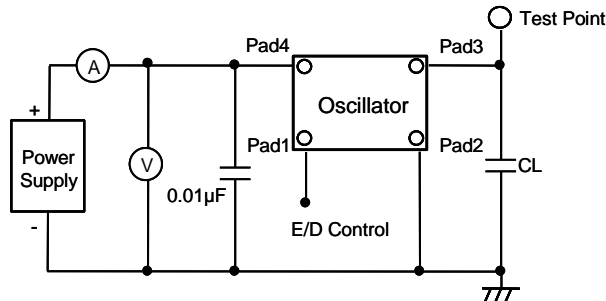
Fig.1 Test Circuits
