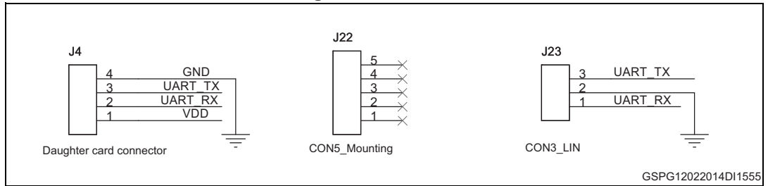
Figure 5. Connector
