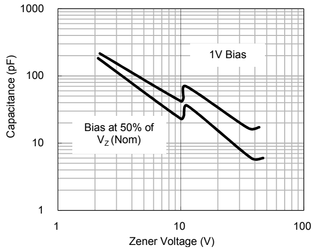
Fig.5 Typical Capacitance
