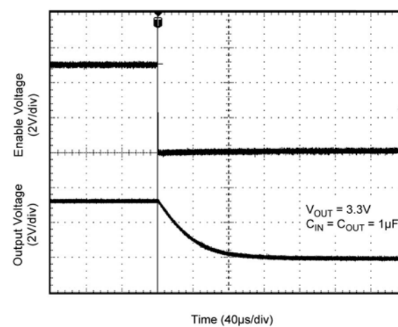
MIC5368 Auto Discharge (No Load)
