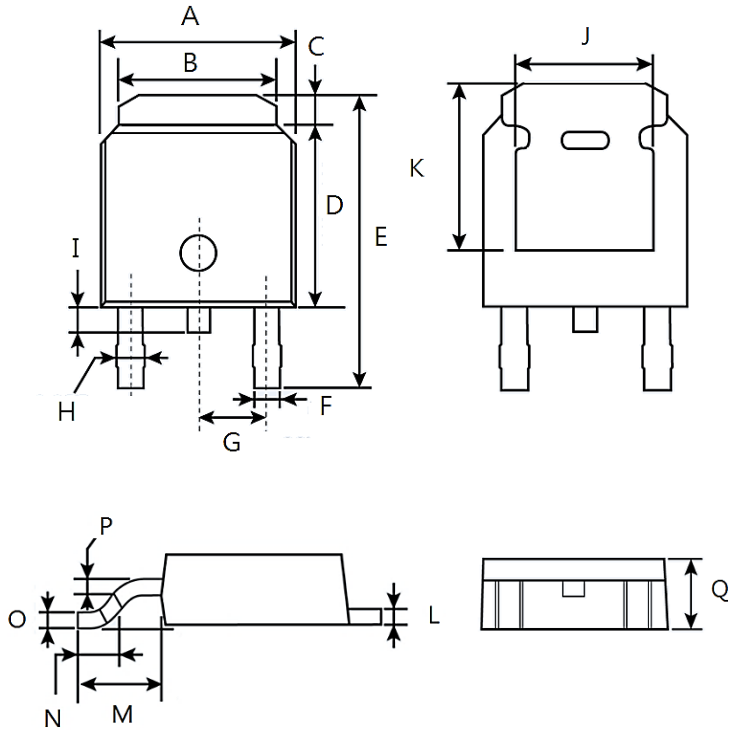
TO-252 (D-PAK)
