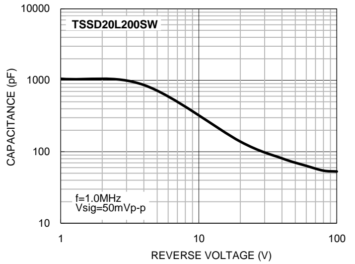
Fig.10 Typical Junction Capacitance
