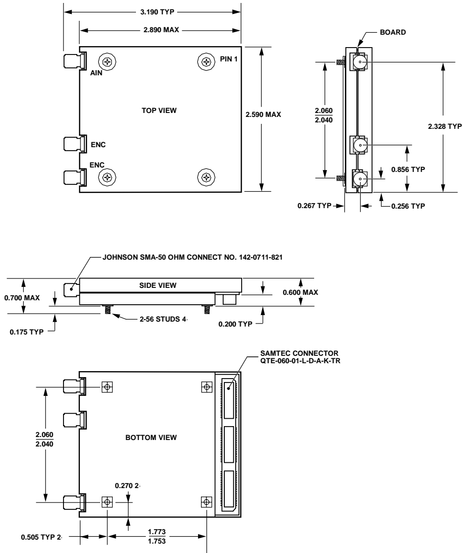
Figure 39. Non-Hermetic Hybrid—Surface-Mounted Parts (WS-Suffix)
