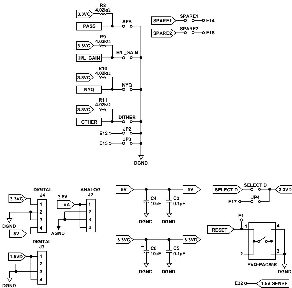
Figure 24. Evaluation Board
