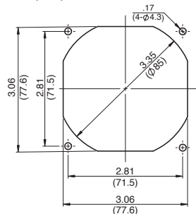
INLET SIDE
