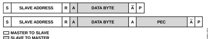
Figure 31. Receive Byte and Receive Byte with PEC
