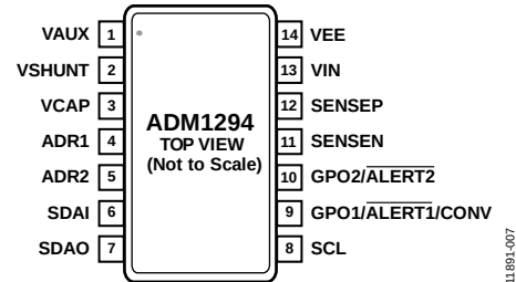
Figure 7. ADM1294 TSSOP Pin Configuration
