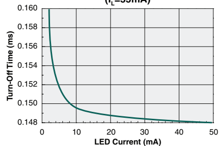
Typical Turn-Off Time vs. LED Forward Current ( I_L = 55\text{mA} )
