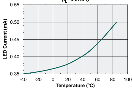
LED Current to Operate vs. Temperature ( I_L = 55\text{mA} )
