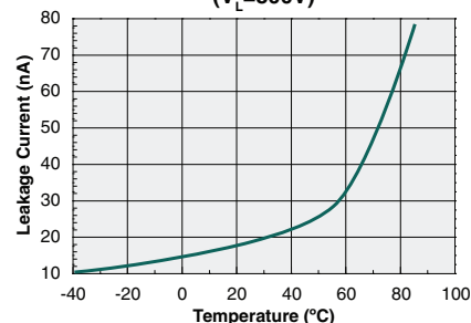
Typical Leakage Current vs. Temperature ( V_L = 800\text{V} )
