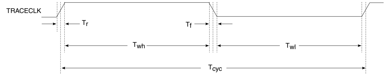
Figure 5. TRACE_CLKOUT specifications
