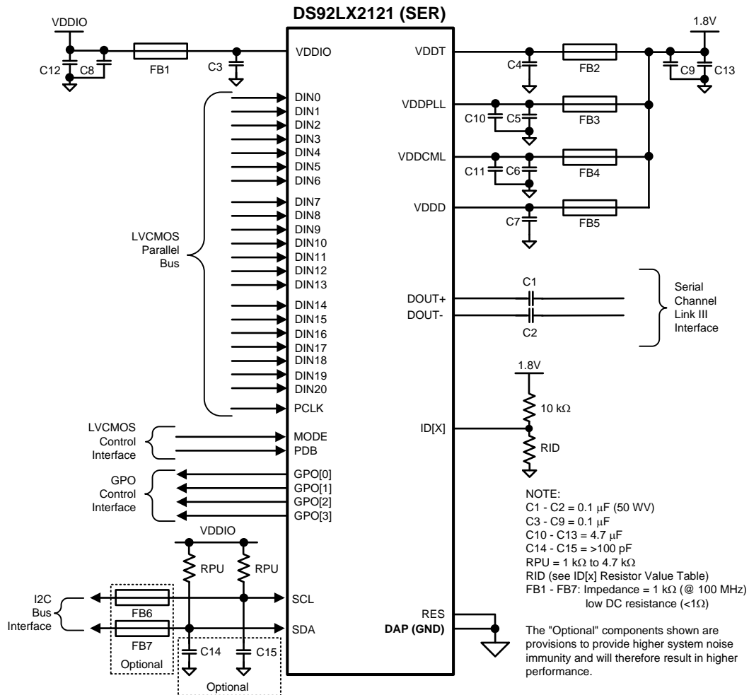
Figure 35. DS92LX2121 Typical Connection Diagram
