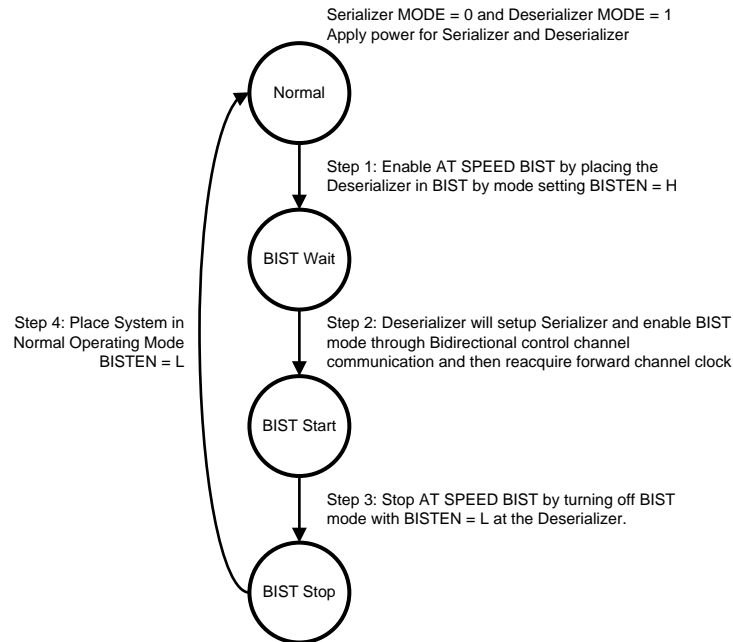
Figure 30. AT-SPEED BIST System Flow Diagram
