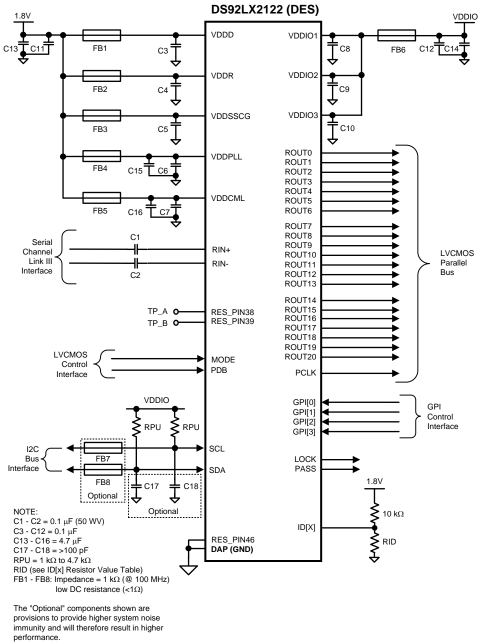
Figure 36. DS92LX2122 Typical Connection Diagram
