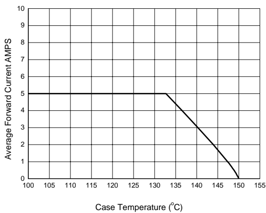
Figure 6. Average Forward Current vs. Case Temperature (Per Diode)
