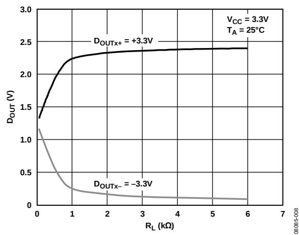
Figure 8. Single-Ended Driver Output Voltage vs. Load Resistance
