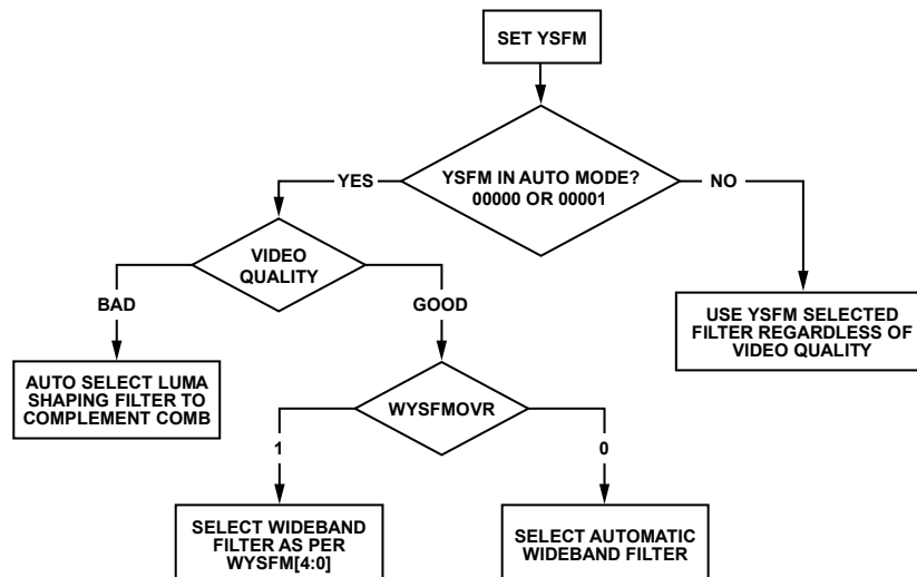
Figure 17. YSFM and WYSFM Control Flowchart
