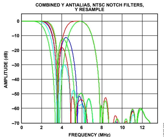
Figure 21. Combined Y Antialias Filter, NTSC Notch Filters
