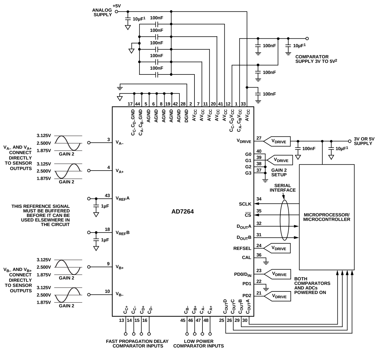
Figure 27. Typical Connection Diagram for the AD7264 in Pin Driven Mode with Gain of 2 and Both ADCs and Comparators Fully Powered On
