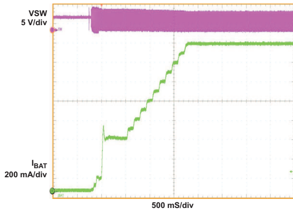
Figure 7. V_{in} = 5\text{V} , V_{BAT} = 3.2\text{V} , No Input Current Limit, I_{CHG} = 1550\text{mA}
