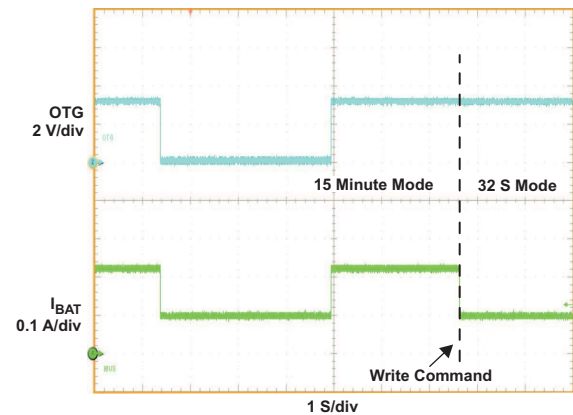
Figure 8. V_{BUS} = 5\text{V} , V_{BAT} = 3.1\text{V} , I_{in\_limit} = 100/500\text{mA} , (OTG Control, 15 Minute Mode), I_{in\_limit} = 100\text{mA} ( I^2\text{C} Control, 32 Second Mode)
