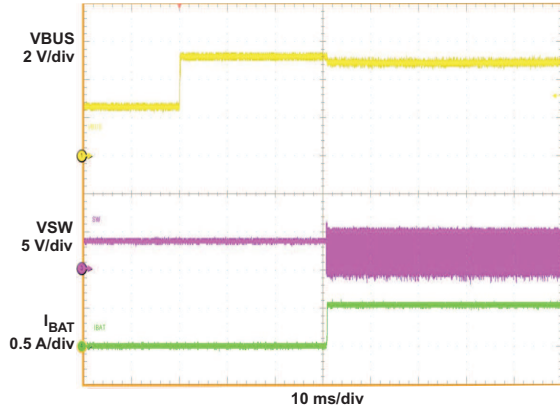
Figure 3. V_{BUS} = 0-5\text{V} , I_{in\_limit} = 500\text{mA} , V_{oreg} = 4.2\text{V} , V_{BAT} = 3.5\text{V} , I_{CHG} = 550\text{mA} , 32S mode
