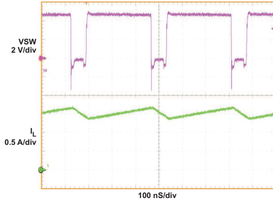
Figure 5. V_{BUS} = 5\text{V} , V_{BAT} = 2.6\text{V} , V_{oreg} = 4.2\text{V} , I_{CHG} = 1550\text{mA}
