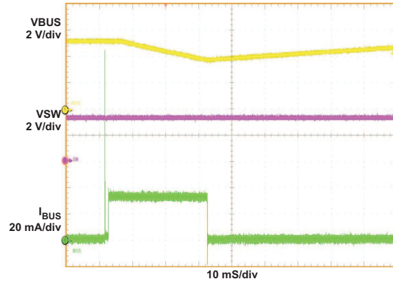
Figure 6. V_{BUS} = 5\text{V} at 8 mA, V_{BAT} = 3.2\text{V} , I_{in\_limit} = 100\text{mA} , I_{CHG} = 550\text{mA}
