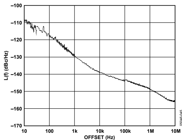
Figure 26. Additive Phase Noise—CMOS DIV 1, 245.76 MHz
