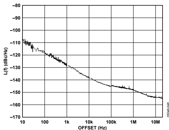
Figure 25. Additive Phase Noise—LVDS DIV 1, 245.76 MHz
