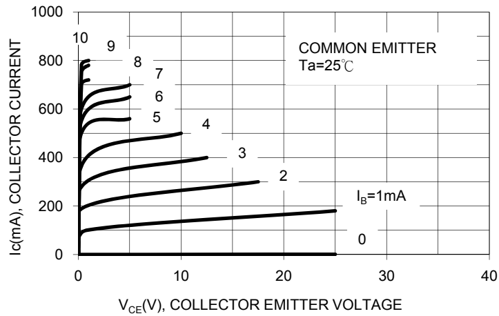
FIG.1 STATIC CHARACTERSTIC
