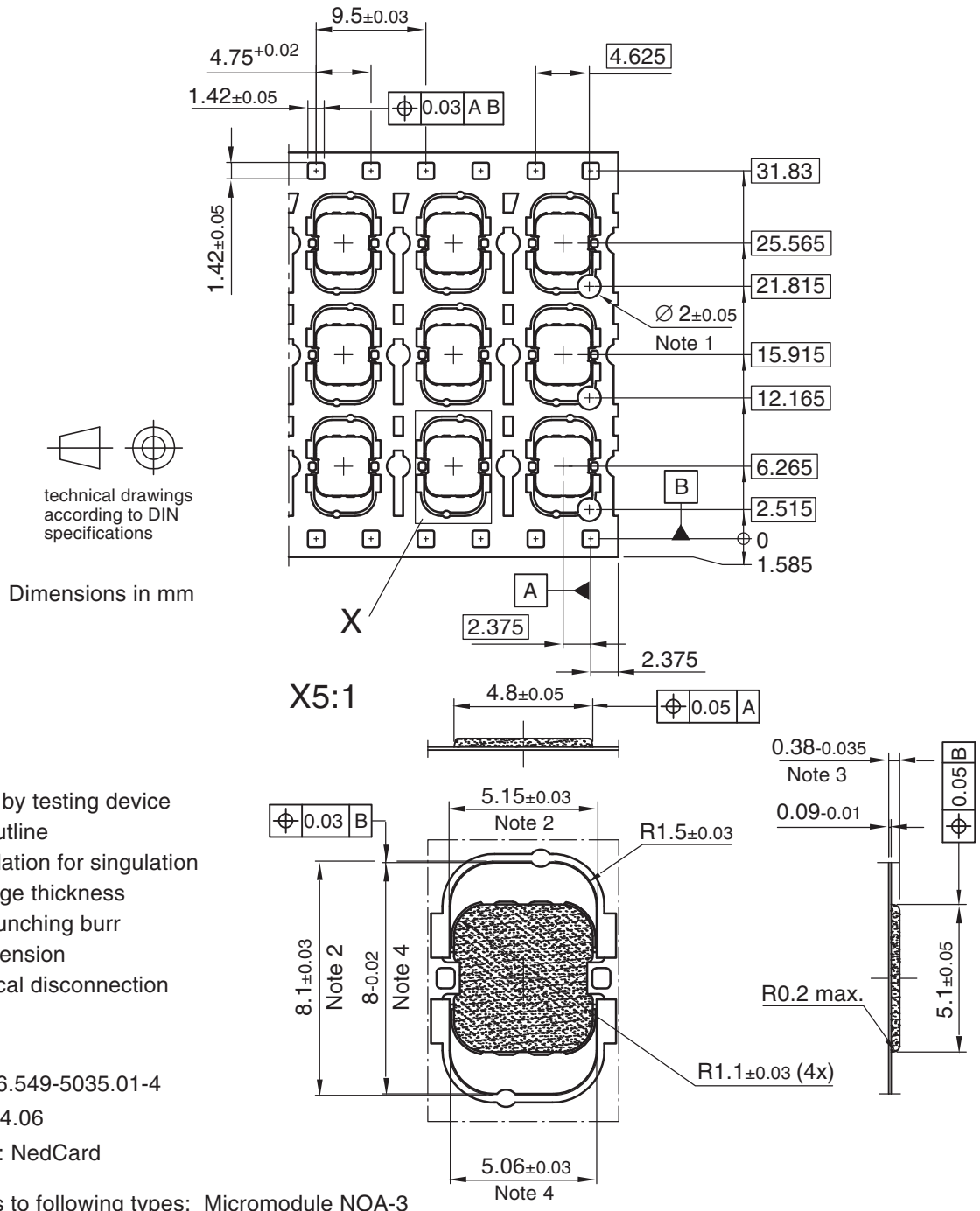
Figure 10-9. NOA3 Micromodule (Planned)
