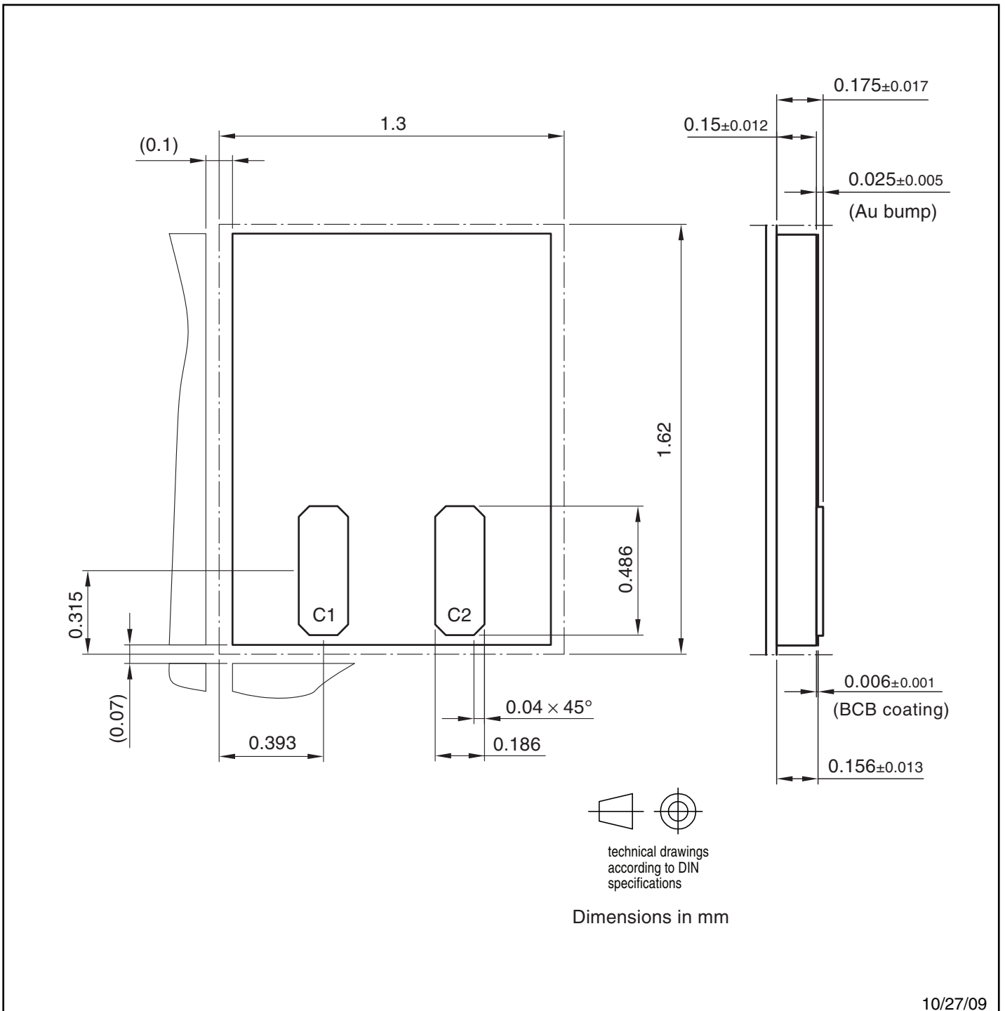
Figure 10-6. Chip Dimensions ATA555812 and ATA555814 Mega Pads with Gold Bumps
