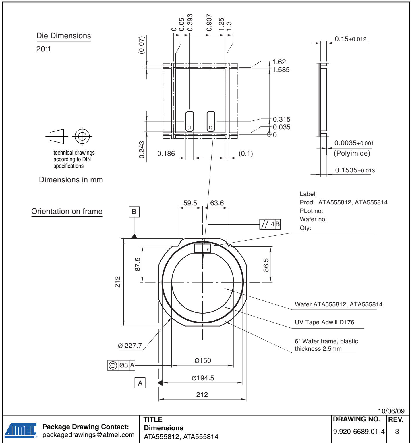
Figure 10-2. 6" Sawn Wafer on Foil with Ring (Type 12/14, Mega Pads)
