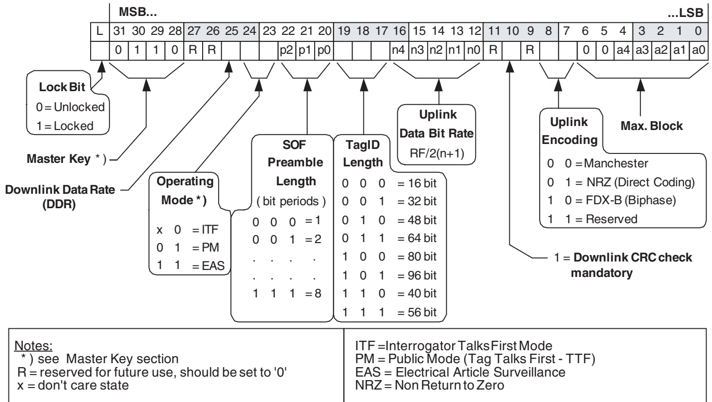
Figure 2-7. Configuration Register
