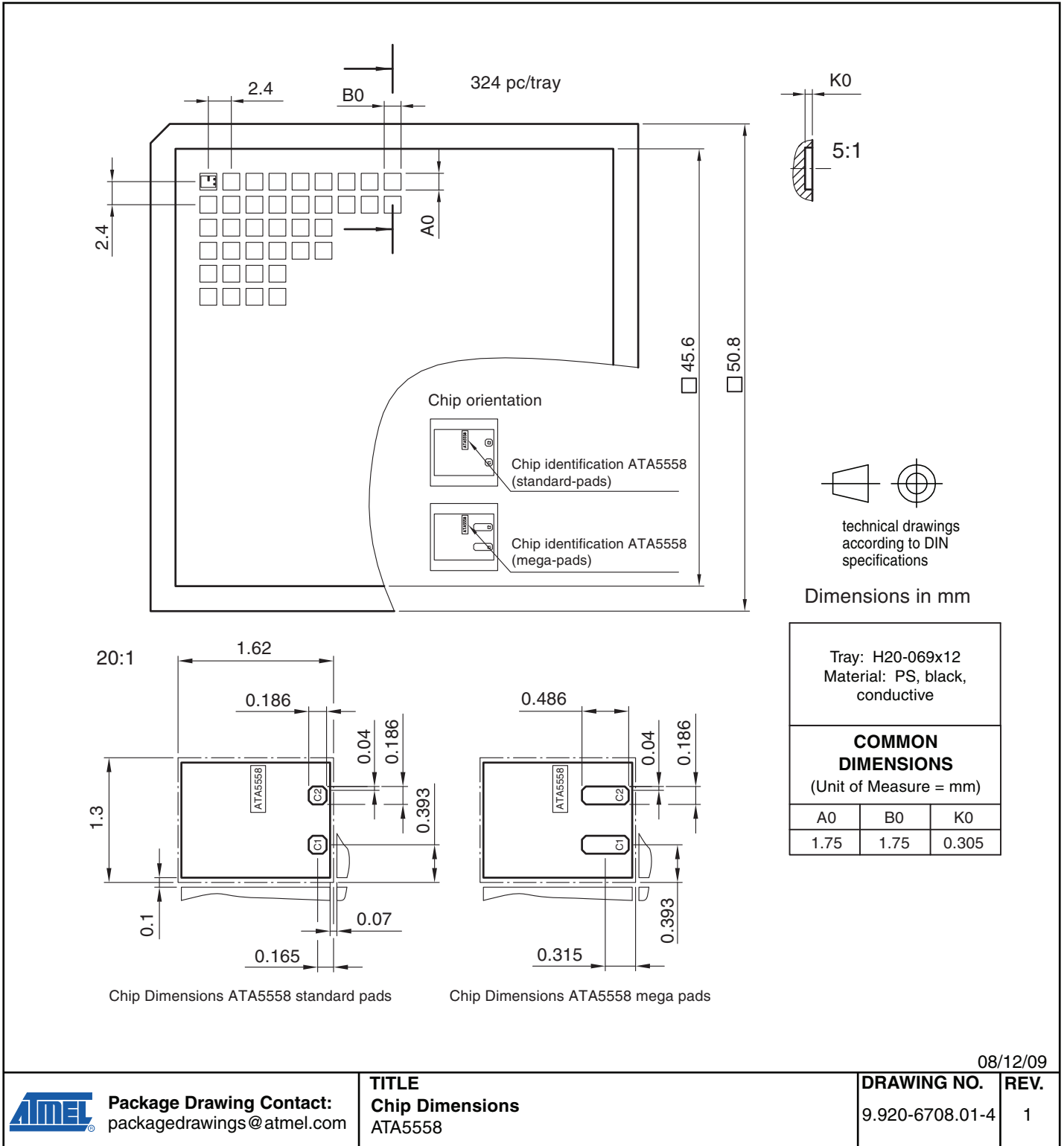
Figure 10-7. Die in Waffle Pack (Type 11 and Type 12/14, Standard Pads, Type 12/14 Mega Pads)
