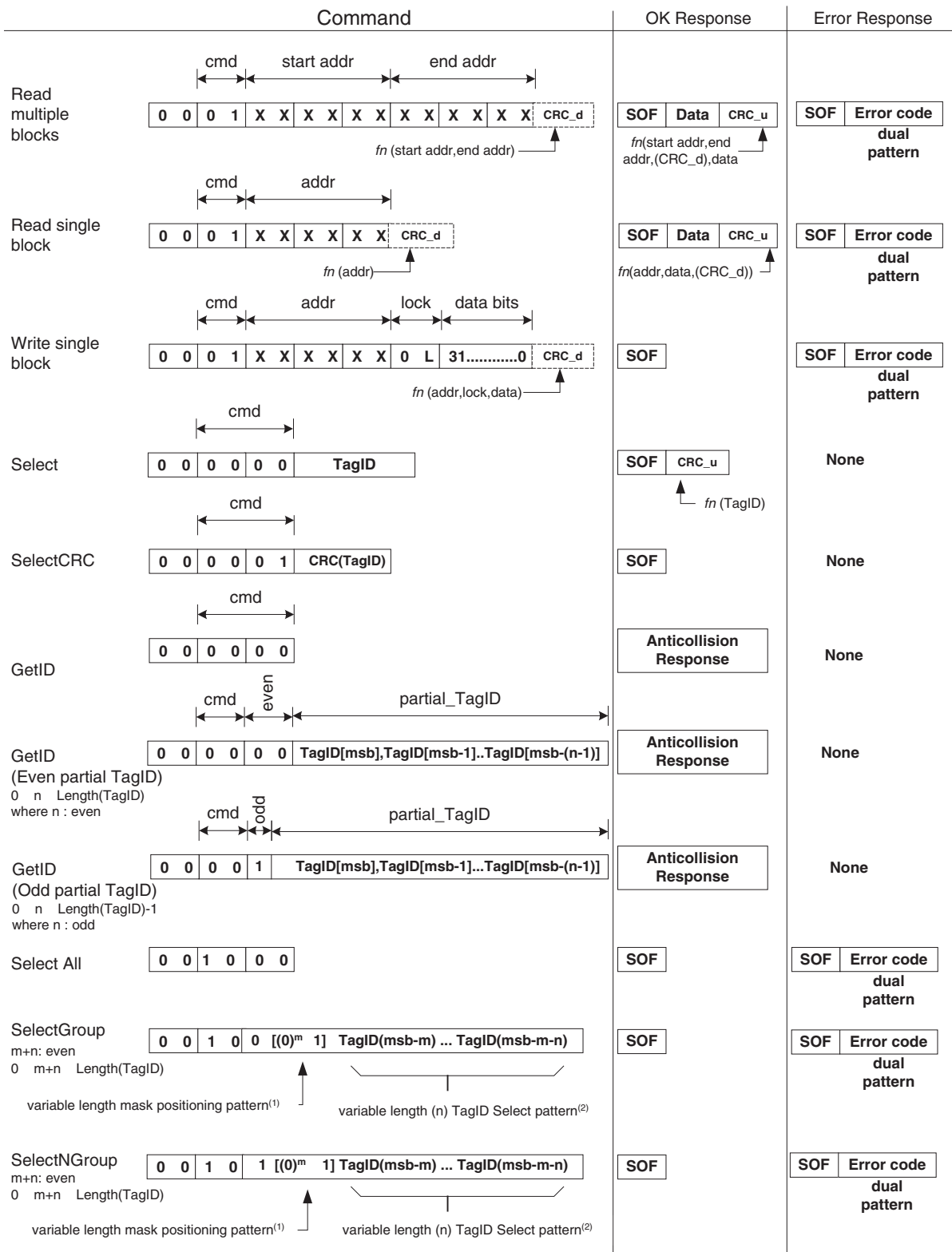
Figure 7-1. Command Format
