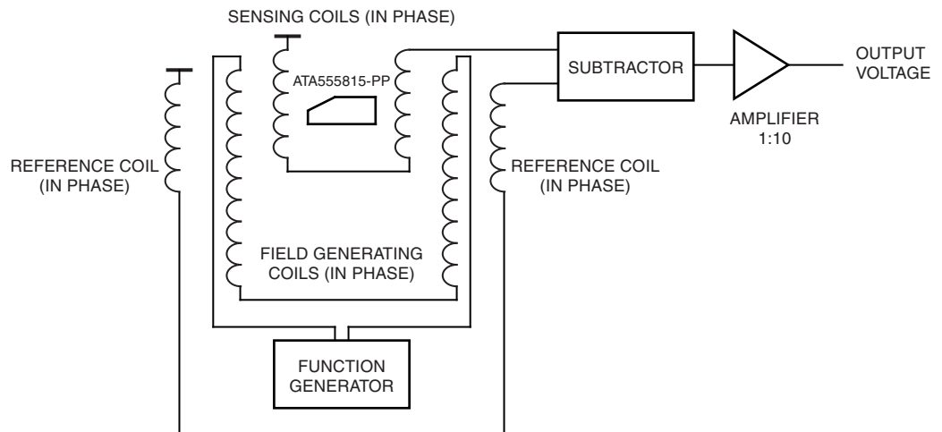
Figure 9-2. Testing Application
