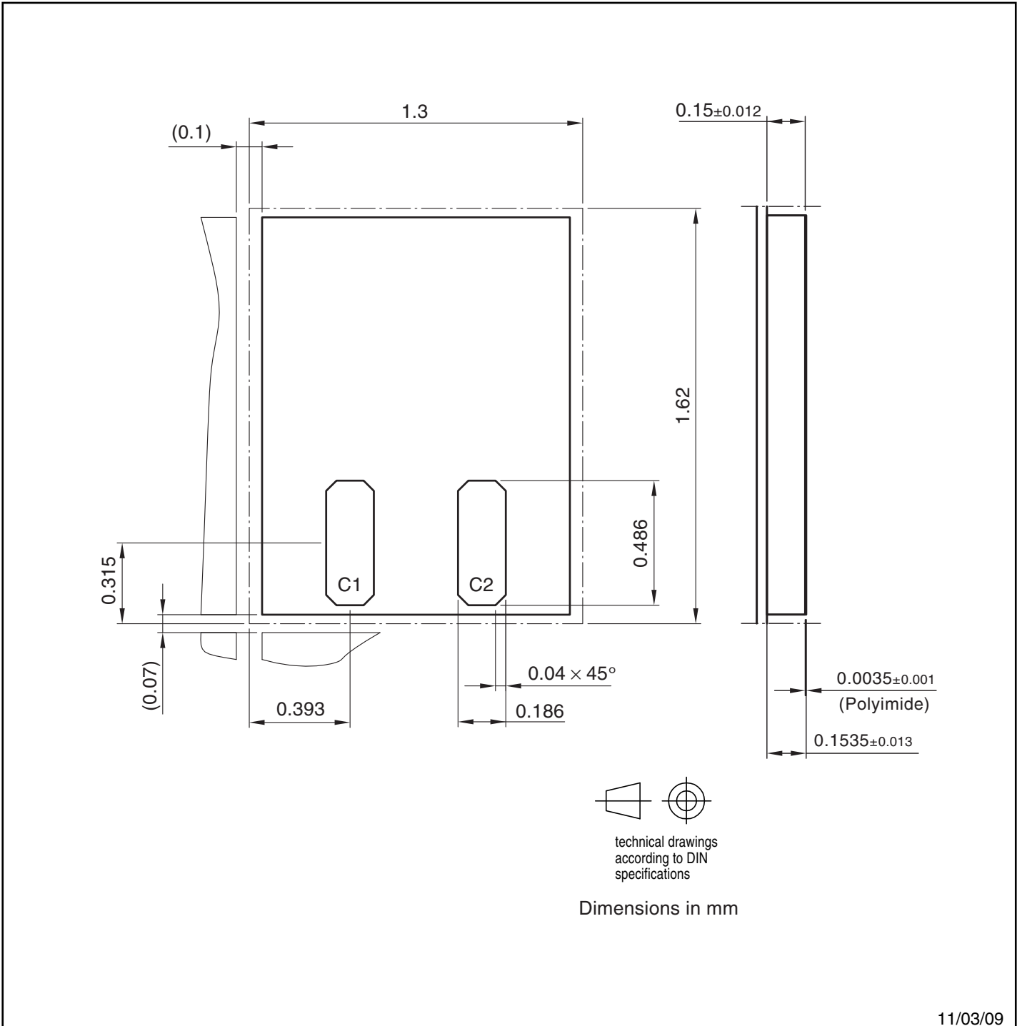
Figure 10-5. Chip Dimensions ATA555812 and ATA555814 Mega Pads
