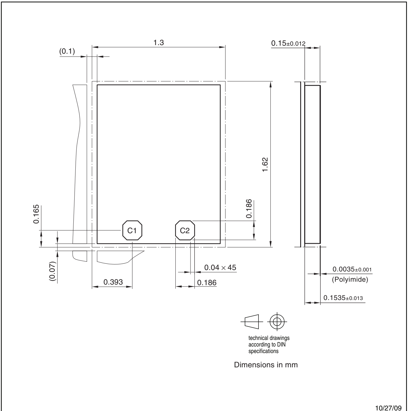
Figure 10-4. Chip Dimensions ATA555811 Standard Pads
