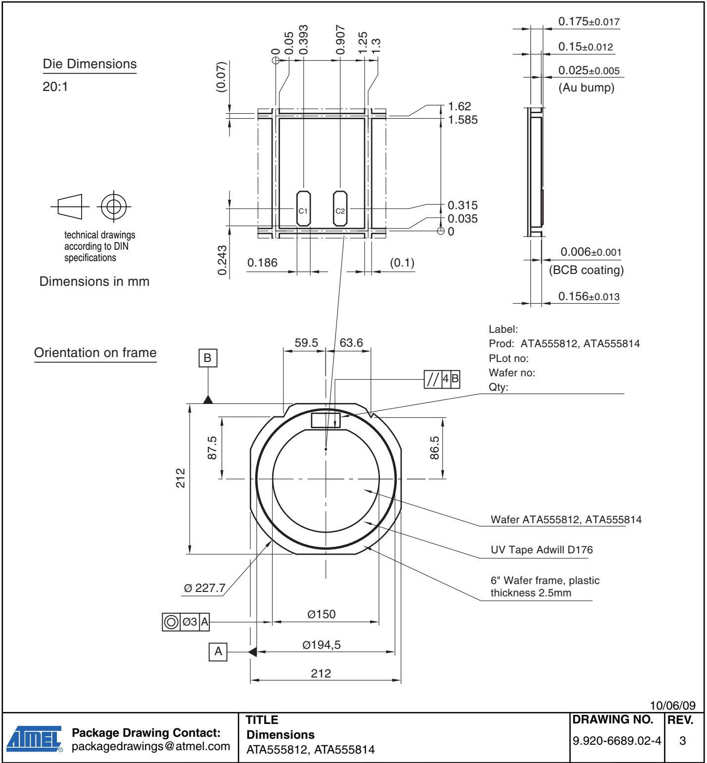
Figure 10-3. 6" Sawn Wafer on Foil with Ring and Goldbumps 25 μm (Type 12/14, Mega Pads)
