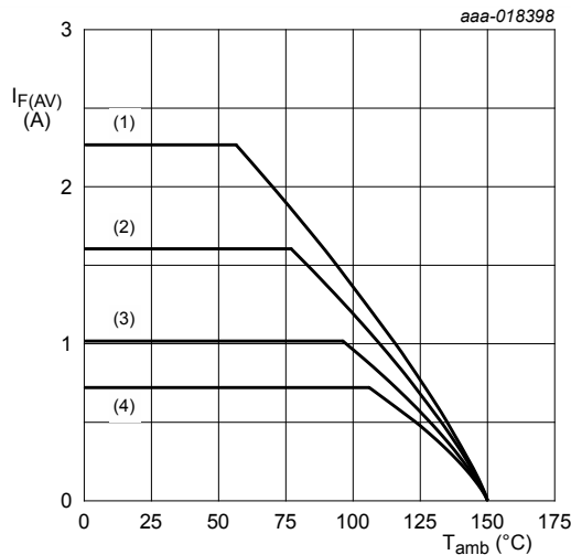
FR4 PCB, standard footprint; one diode loaded (1) \delta = 1 (2) \delta = 0.5 (3) \delta = 0.2 (4) \delta = 0.1
