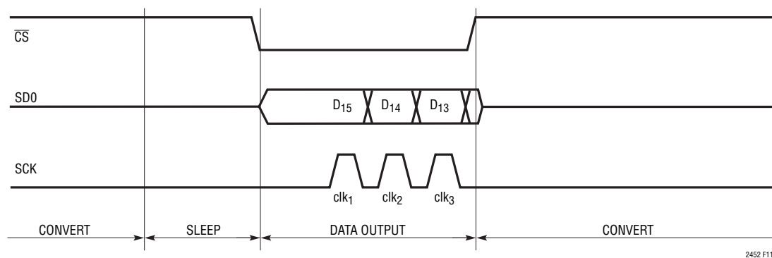
Figure 11. Idle-Low (CPOL = 0) Clock and Aborted I/O Example
