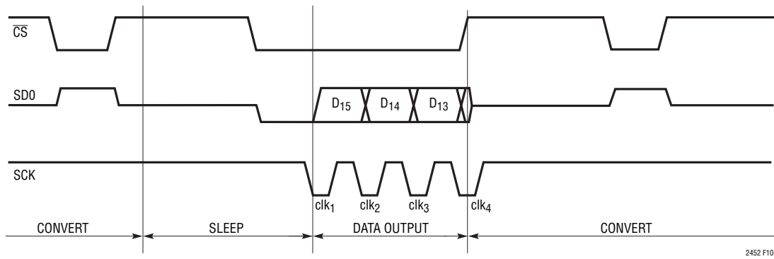
Figure 10. Idle-High (CPOL = 1) Clock and Aborted I/O Example
