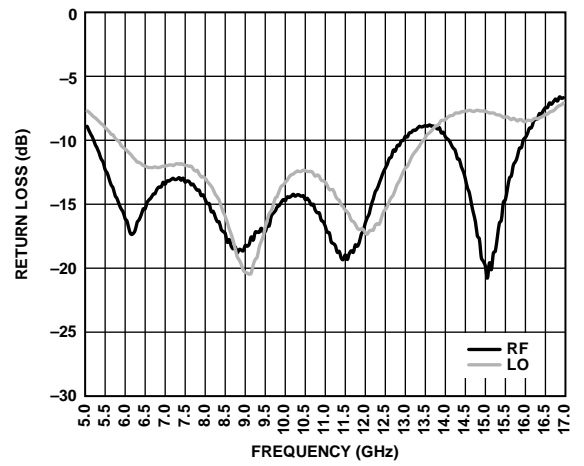
Figure 79. Return Loss vs. Frequency, LO = 0 dBm at 10 GHz, TA = 25°C
