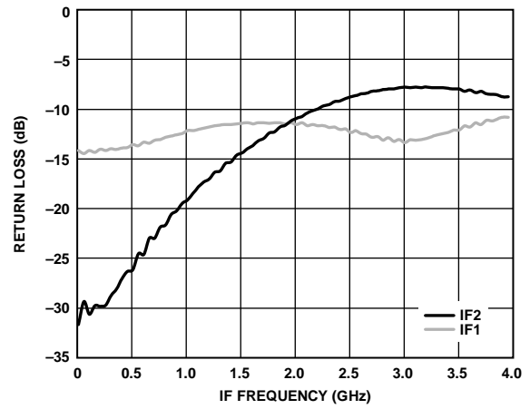
Figure 78. Return Loss vs. IF Frequency, LO = 17 dBm, TA = 25°C
