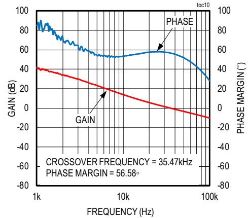
BODE PLOT V_{IN} = 24V , V_{OUT} = 6.3V , FULL LOAD, PWM MODE
