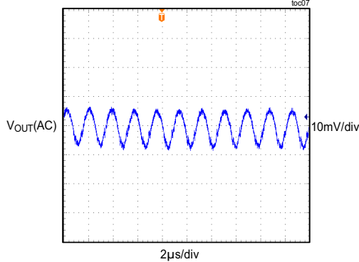
OUTPUT VOLTAGE RIPPLE V_{IN} = 24V , V_{OUT} = 6.3V , FULL LOAD, PWM MODE
