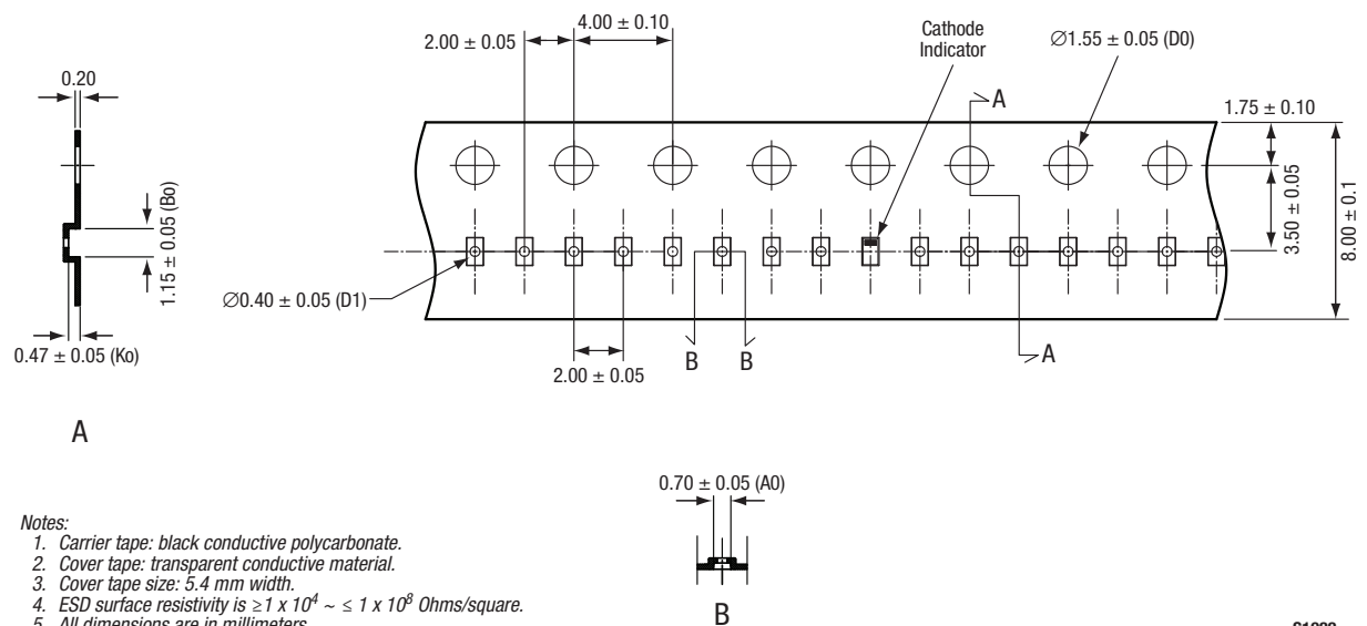
Figure 10. SOD-882 Tape and Reel Dimensions
