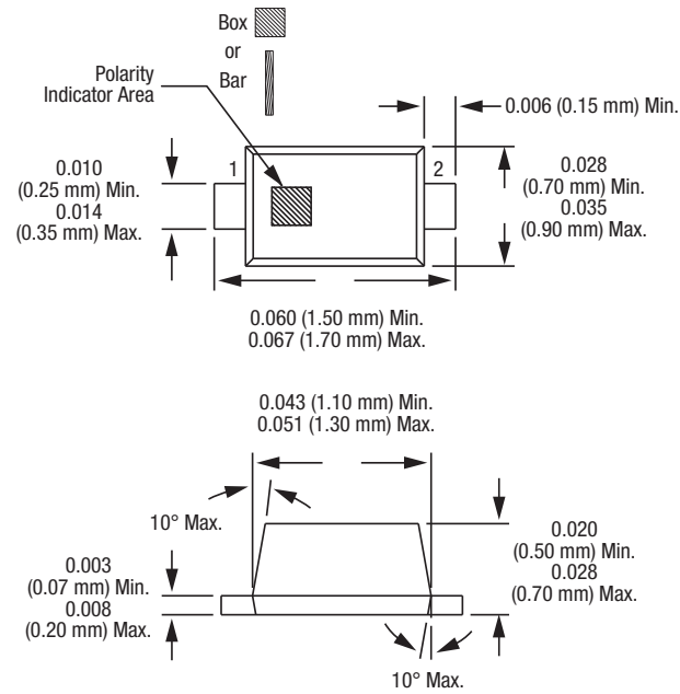
Figure 5. SC-79 Package Dimensions
