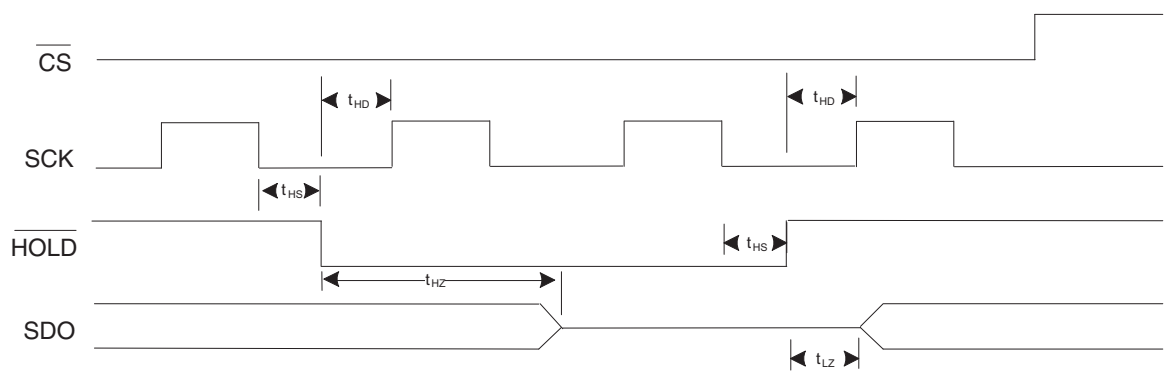
Figure 4-2. Hold Timing
