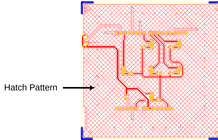
Figure 2-10: Hatch Pattern on Bottom Layer of Board
