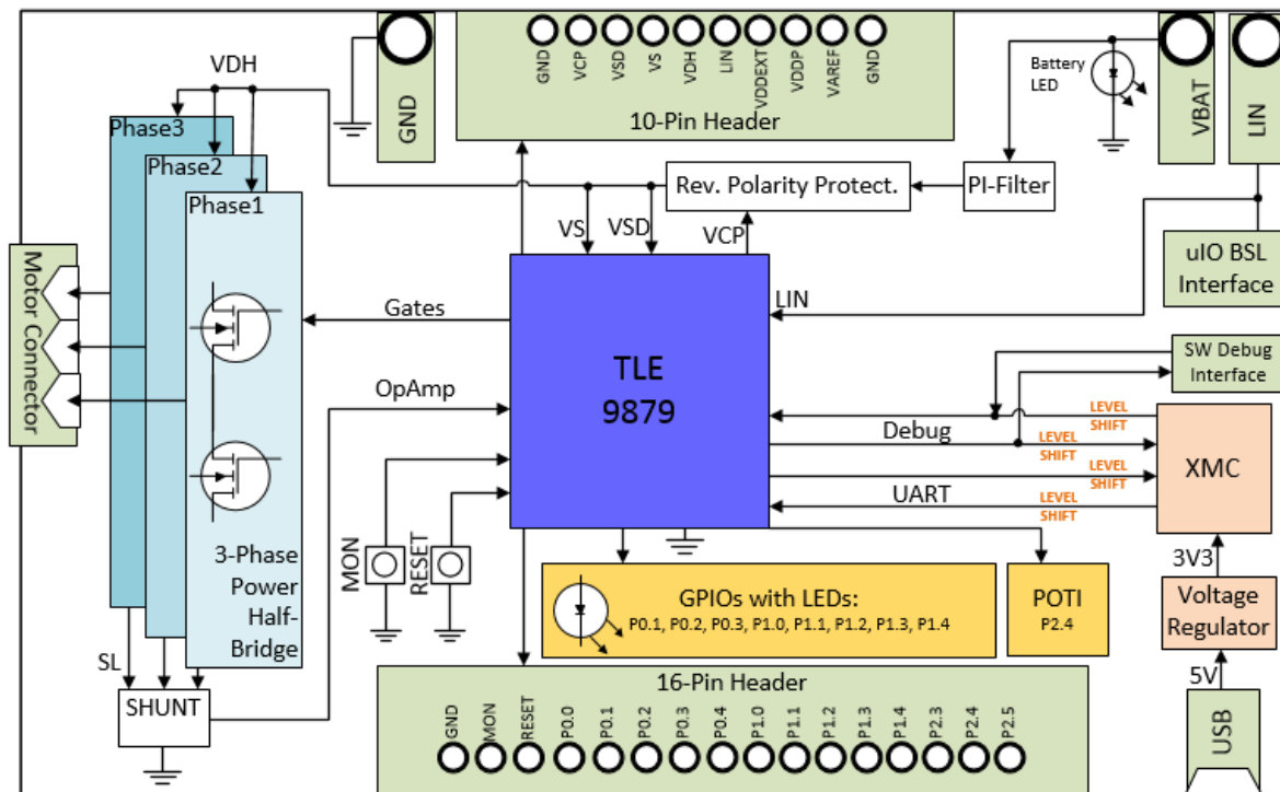
Figure 1: Board Concept
