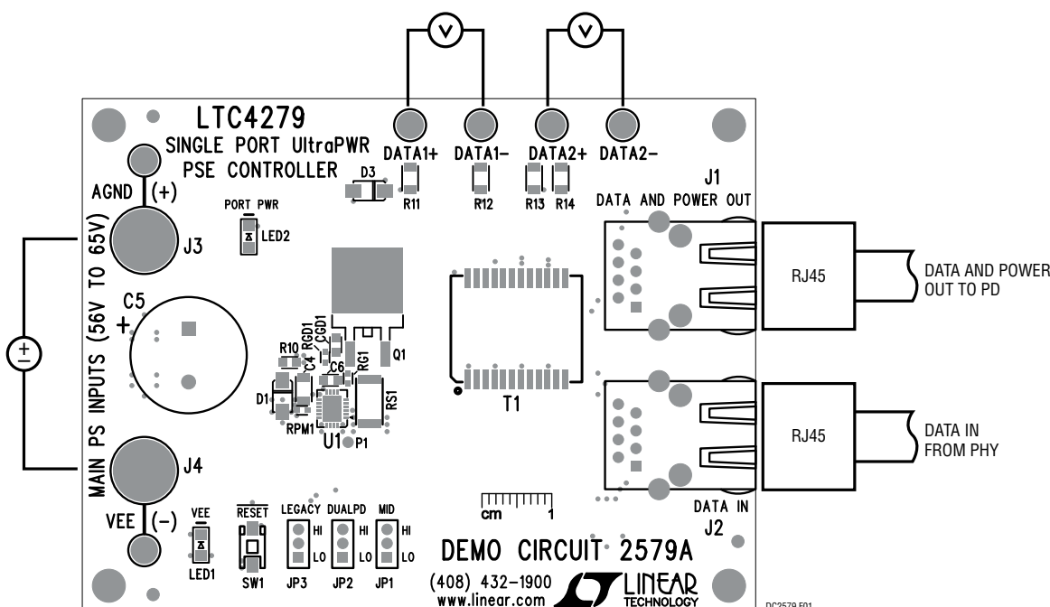
Figure 1. DC2579A Connections
