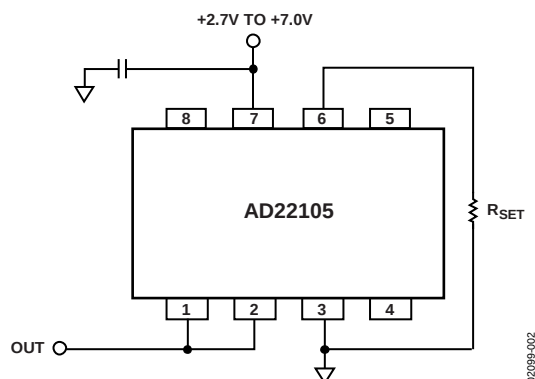
Figure 14. Typical Application Circuit
