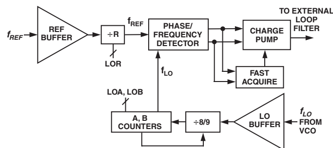
Figure 5. LO Synthesizer
