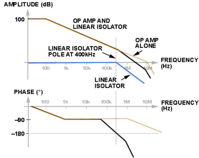
Figure 6. Bode Plot 1
