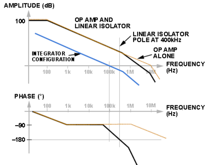
Figure 7. Bode Plot 2
