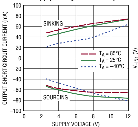
Output Short-Circuit Current vs Supply Voltage, Either Output
