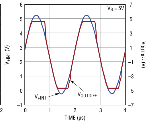
Overdrive Recovery
