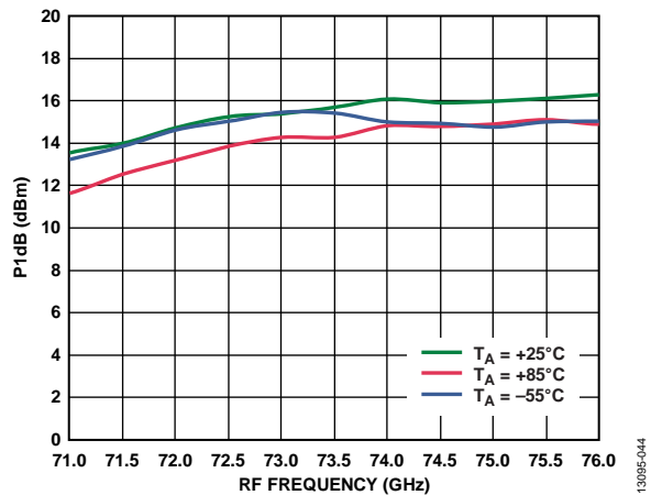
Figure 43. Input P1dB vs. RF Frequency at Various Temperatures, LO = 2 \text{ dBm} , IF = 2000 \text{ MHz} , LSB
