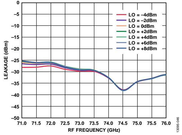
Figure 45. 6 \times LO Leakage at RFOUT vs. RF Frequency at Various LO Powers, I_{FIN} = 5 \text{ dBm} , IF = 2000 \text{ MHz} , LSB
