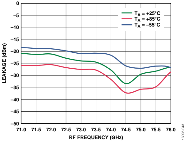
Figure 42. 6 \times LO Leakage at RFOUT vs. RF Frequency at Various Temperatures, I_{FIN} = 5 \text{ dBm} , LO = 2 \text{ dBm} , IF = 2000 \text{ MHz} , LSB
