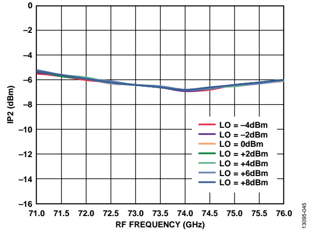
Figure 44. Input IP2 vs. RF Frequency at Various LO Powers, I_{FIN} = 5 \text{ dBm} , IF = 2000 \text{ MHz} , LSB
