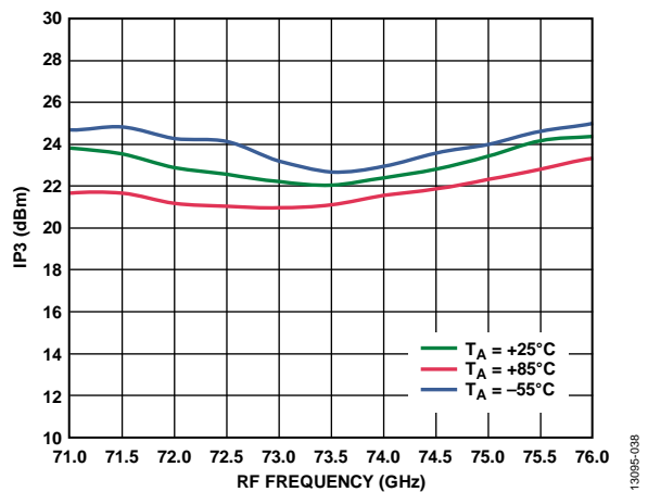
Figure 37. Input IP3 vs. RF Frequency at Various Temperatures, I_{FIN} = 5 dBm, LO = 2 dBm, IF = 2000 MHz, LSB
