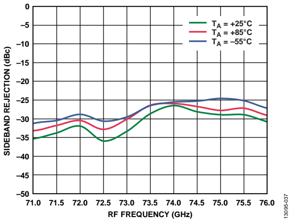
Figure 36. Sideband Rejection vs. RF Frequency at Various Temperatures, I_{FIN} = -8 dBm, LO = 2 dBm, IF = 2000 MHz, LSB
