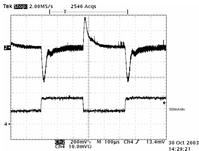
Figure 7. DC533 Step Load Response ( I_{OUT} = 400\text{mA} to 800\text{mA} , V_{IN} = 5\text{V} , T_A = 25^\circ\text{C} , V_{OUT} = 12\text{V} ) CH2 is V_{OUT} ripple (AC), CH4 is I_{OUT} (500mA/10mV \Omega )
