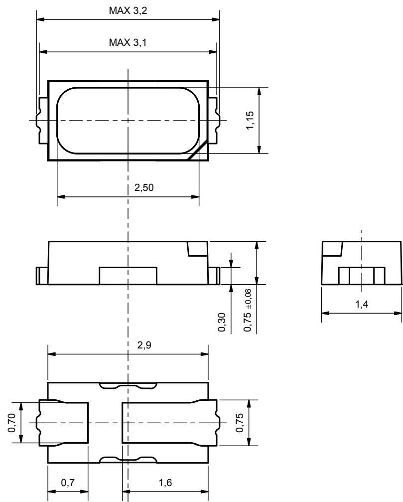
Figure 8. Mechanical dimensions for LUXEON 3014.
