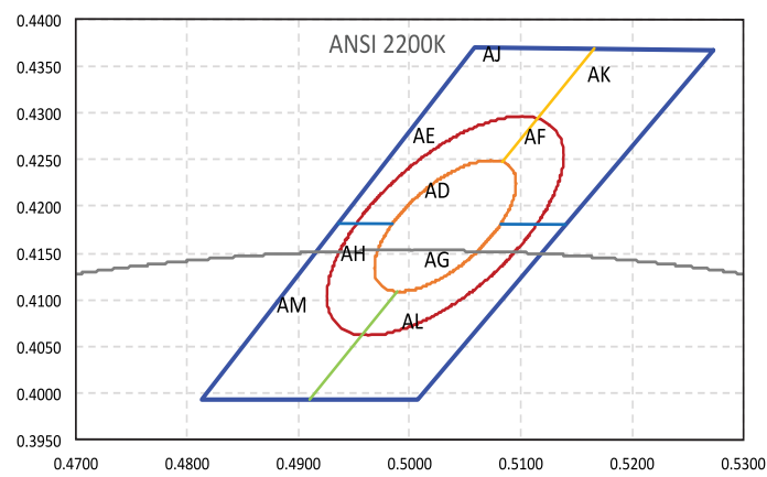
Figure 7a. Color bin structure for LUXEON 3014 2200K, hot-color targeted at T j =65°C.
