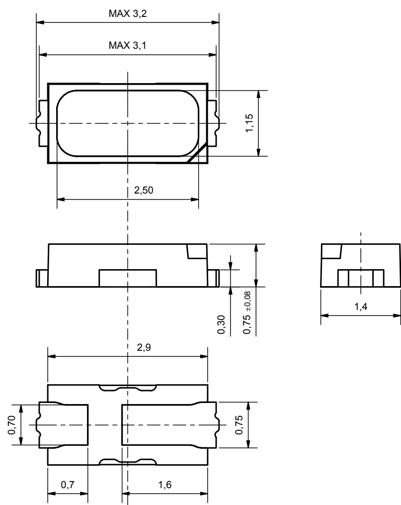
Figure 8. Mechanical dimensions for LUXEON 3014.
