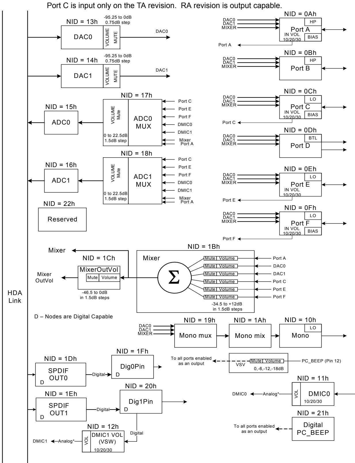
Figure 9. Widget Diagram
