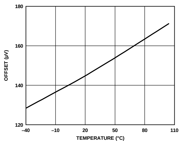
Figure 8. Offset vs. Temperature
