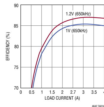
Efficiency vs Load Current at 12V input
