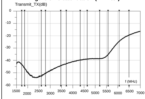
Figure 8: fo attenuation (TX filter)
